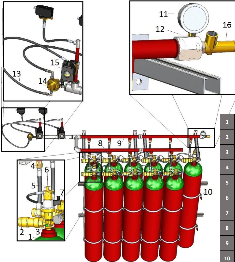
Selector Valve System
