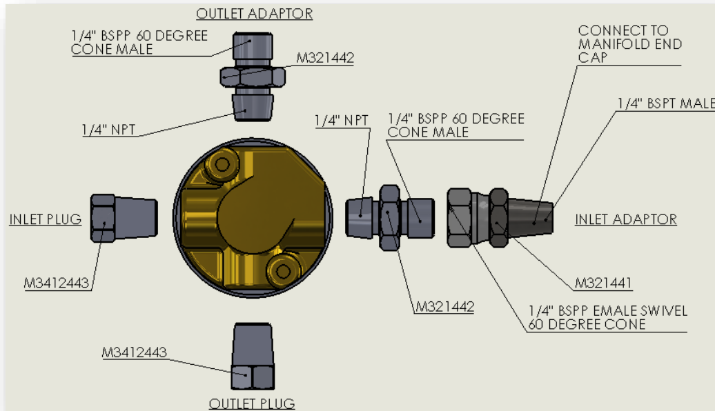
Connection Details
