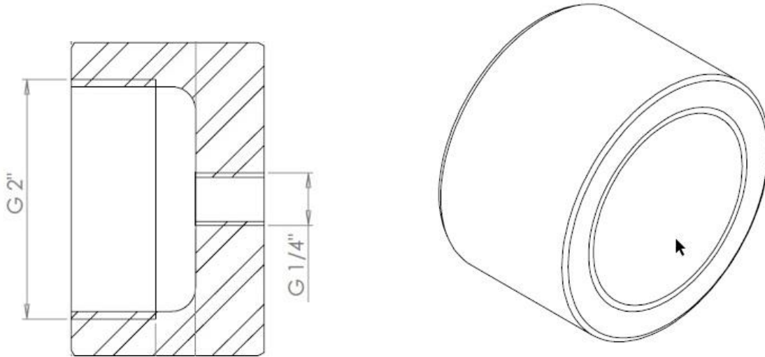
End cap size and connection threads
